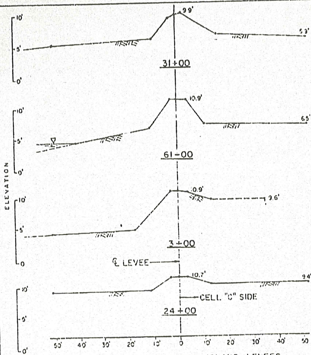
SECTIONS THRU ALEXANDER ISLAND LEVEES
